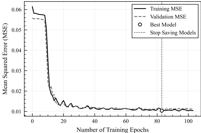
Learning Curve of TCSEA-Transformer Model for SolarPlant-1 (Gyeongju)
